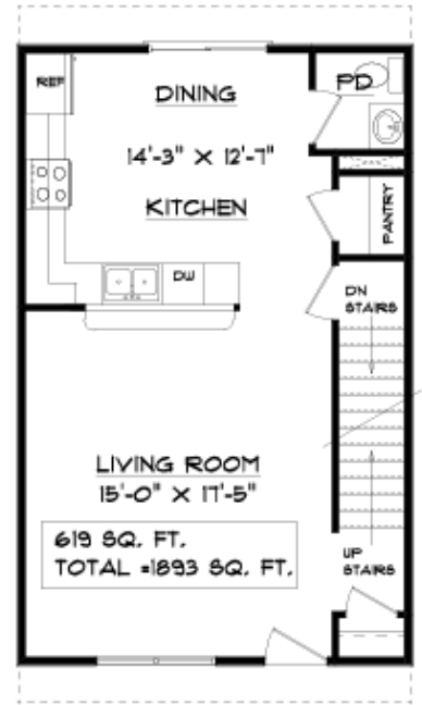
1ST FLOOR
